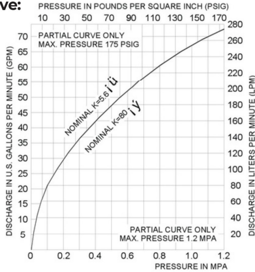
FIGURE B : NOMINAL DISCHARGE CURVE
